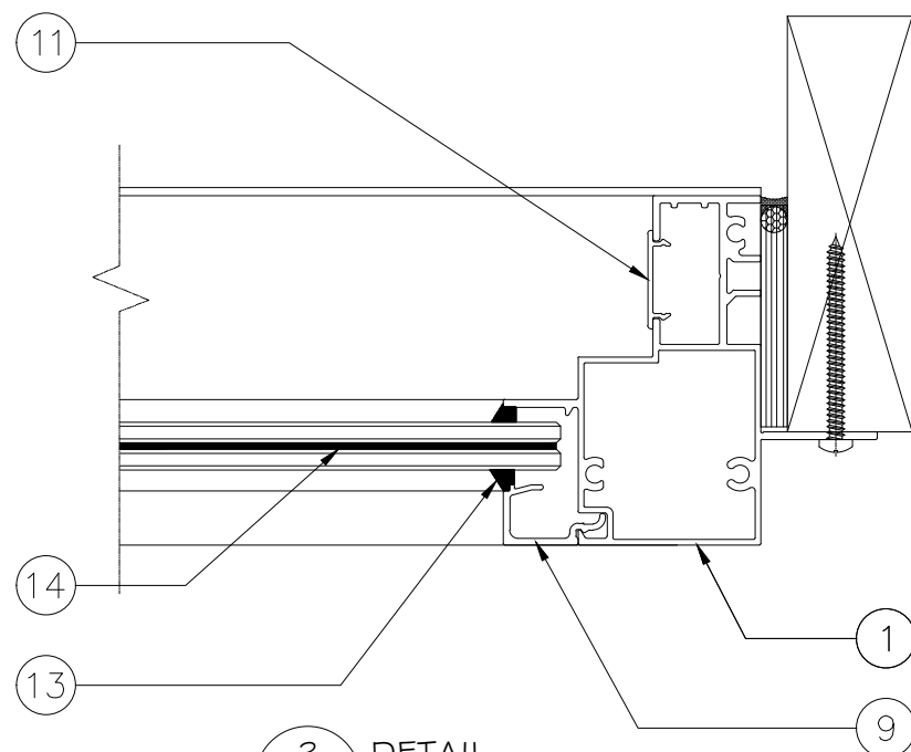
3 DETAIL D4
