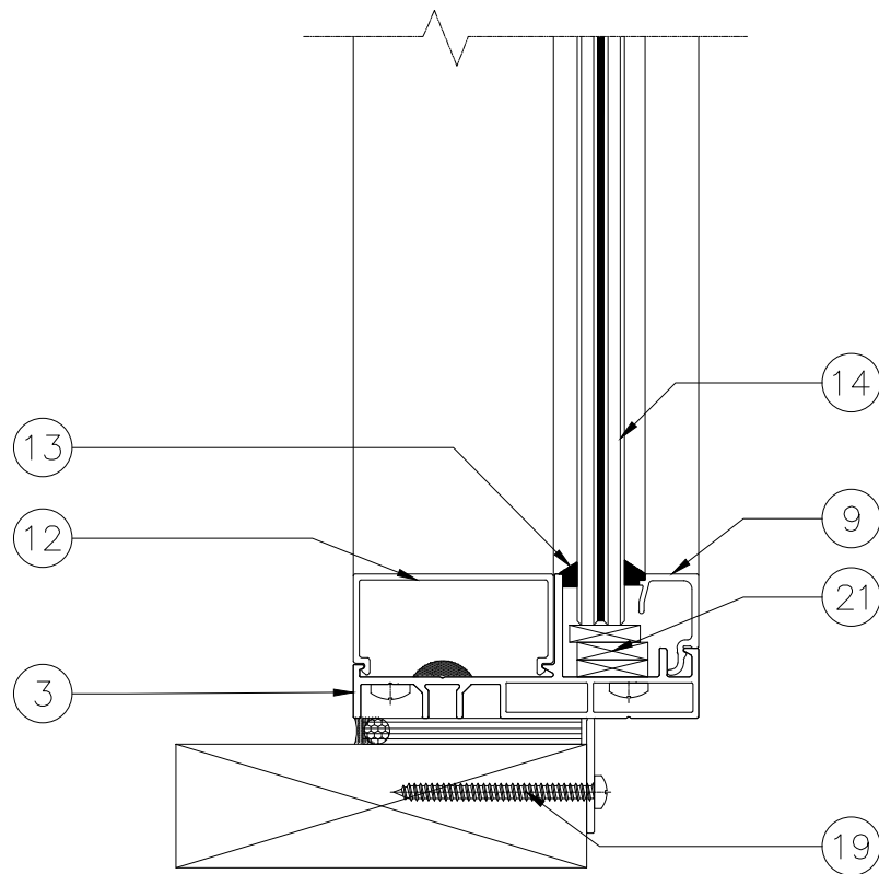
2 DETAIL D4
