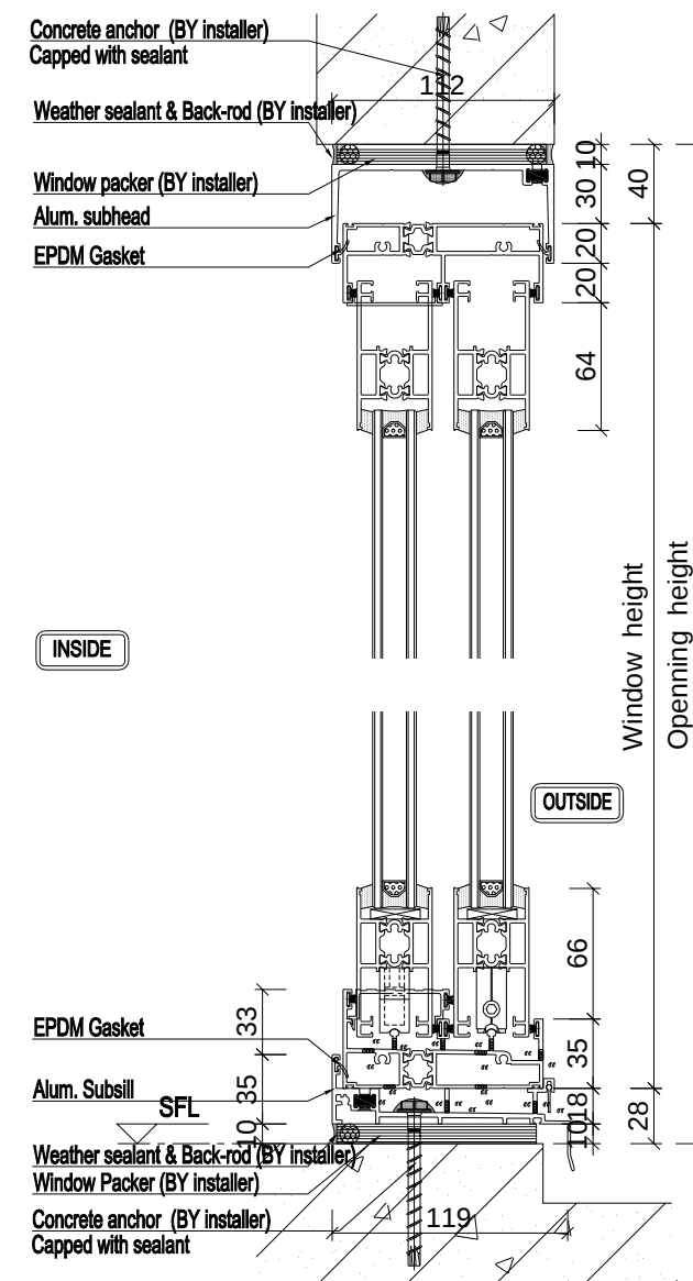
Section 1-1
