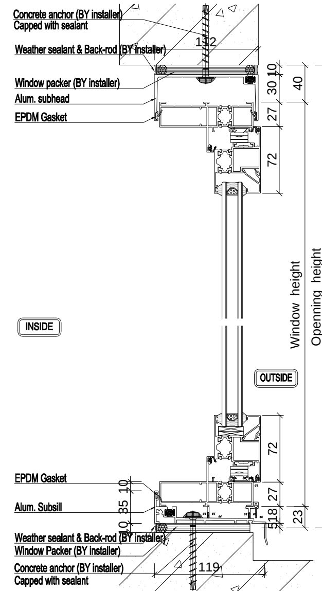
Section 1-1
